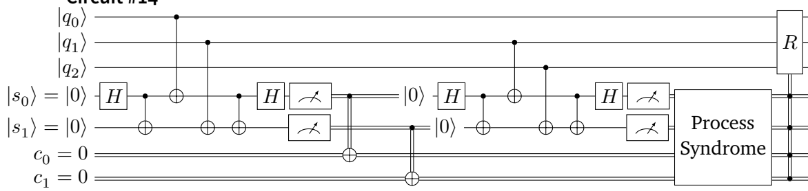
Circuit #14
