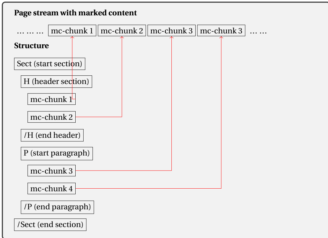
Figure 2: Schematic description of the relation between marked content in the page stream and the structure
